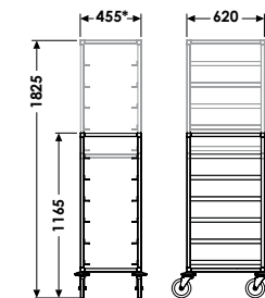
Gastronorm, *Euronorm: +45 mm
